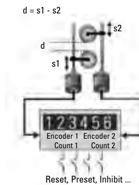
Difference-Position display
