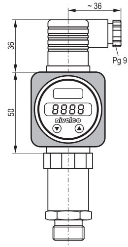
D□□ - 4□□ - □ Flush diaphragm pipe coupling
