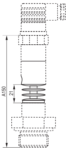
D□C - 4□□ - □ Inner st. st. diaphragm 1/2" Flush diaphragm
